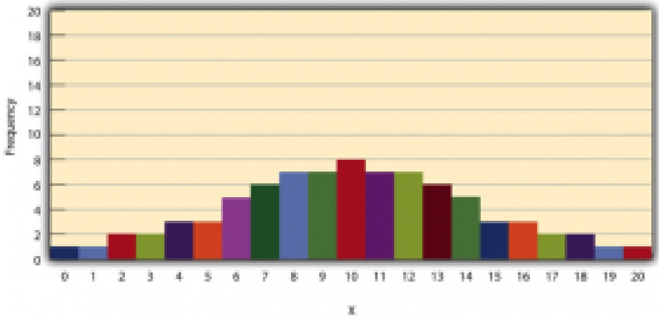
Figure 12.4 Histograms Showing Hypothetical Distributions With the Same Mean, Median, and Mode (10) but With Low Variability (Top) and High Variability (Bottom). [Image description]
