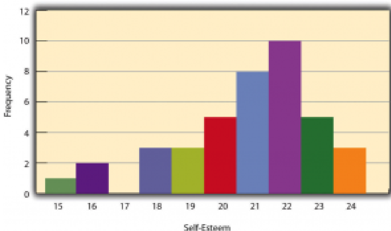
Figure 12.1 Histogram Showing the Distribution of Self-Esteem Scores Presented in Table 12.1
