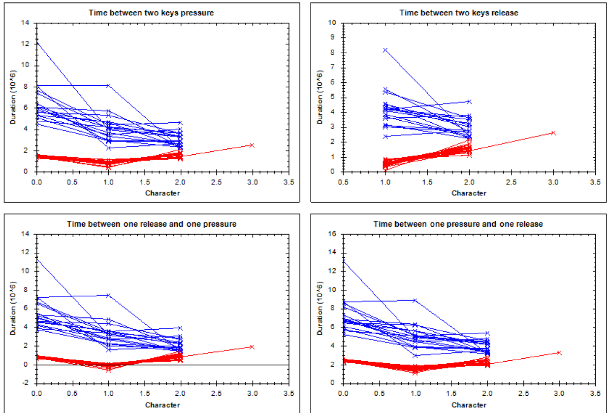
Figure 4.7: Gray Keystroke Dynamics (Action Based Authentication)
