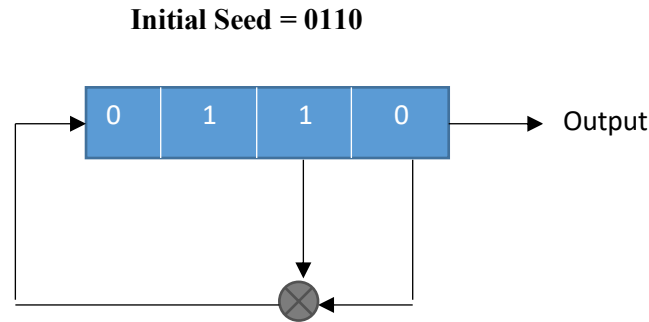
Figure 6.9: LFSR Using four (4) Registers
