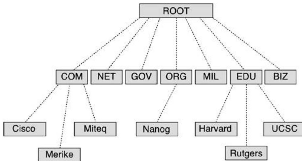
Fig. 2.6: DNS Hierarchy
