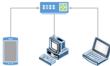
Fig. 1.1: Intranet Example
