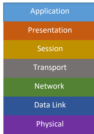
Fig. 2.3: OSI Model
