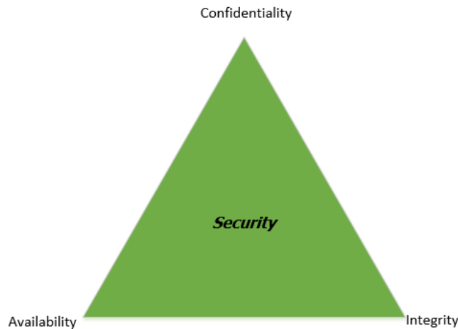
Fig. 1.3: CIA Triangle
