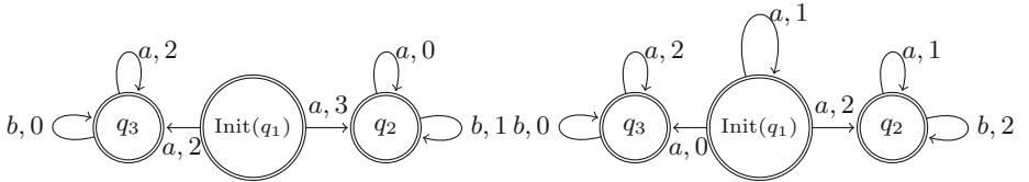
Fig. 2. Weighted automaton P
