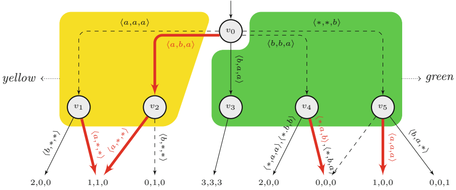
Fig. 1. An example of a concurrent game with public signal (yellow and green: public signal). Edges in red and bold are part of the strategy profile. Dashed edges are the possible deviations. One can notice that none of the deviations is profitable to the deviator, hence the strategy profile is a Nash equilibrium. Convention in the drawing: edges with no label are for complementary labels (for instance the edge from v_5 to 0,0,0 is labelled by all \langle a_1, a_2, a_3 \rangle not in the set \{\langle a, a, a \rangle, \langle b, a, a \rangle, \langle b, a, b \rangle\} (Color figure online))
