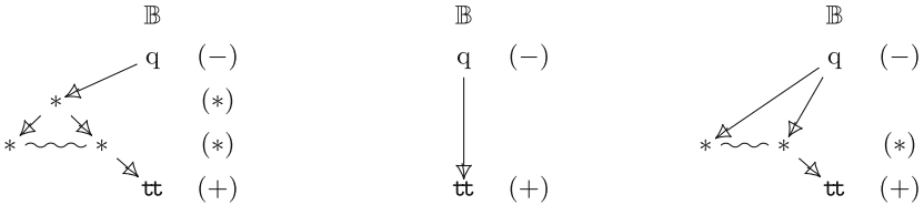
(a) Interp. before hiding (b) Interp. after hiding (c) Interp. with partial hiding
