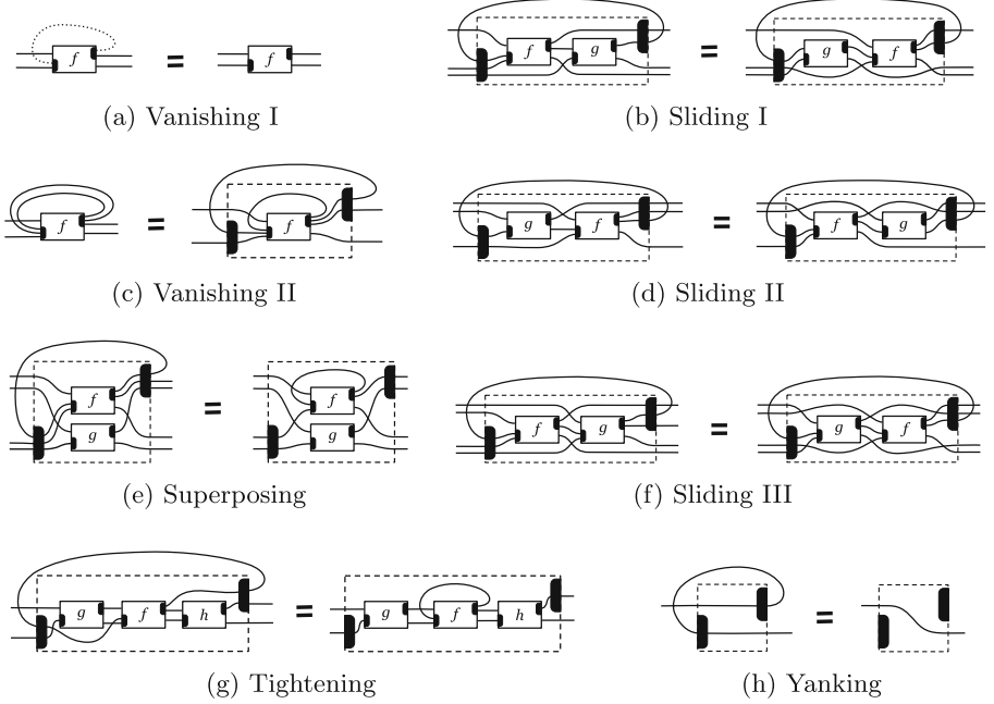
Fig. 4. Axioms of guarded traced categories
