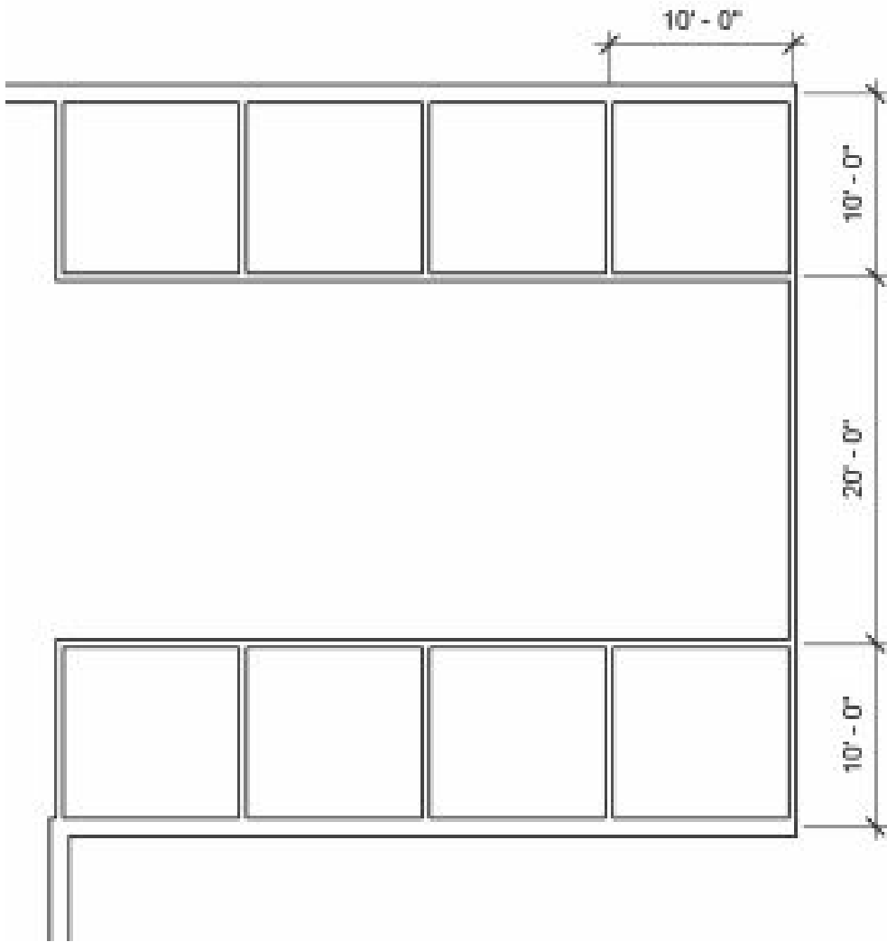
Figure 2.25 Eight enclosed rooms with dimension lines
