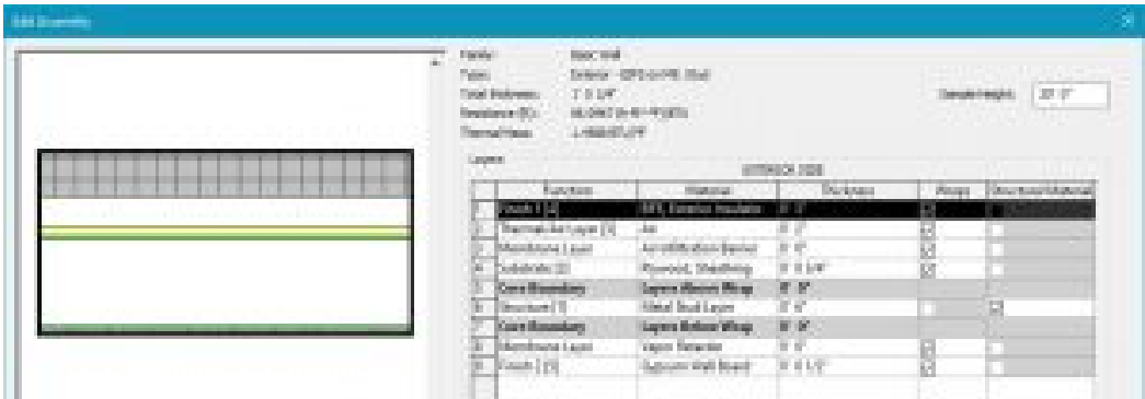
Figure 2.10 Basic Wall Exterior – EIFS on Mtl. Stud
