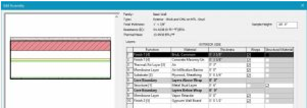
Figure 2.6 Basic Wall Exterior – Brick on CMU on MTL Stud
