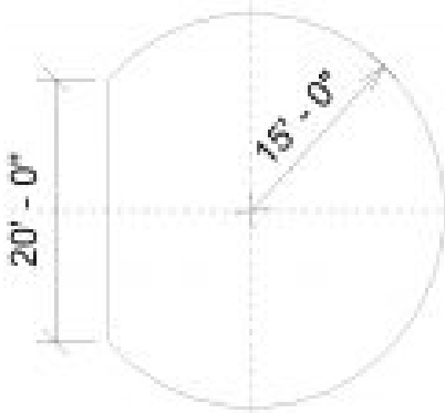
Figure 6.6 Conceptual mass shown with dimensions in plan view and in 3D view
