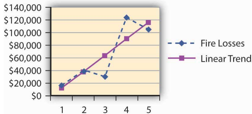
Figure 4.6 Linear Regression Trend of Losses of A
