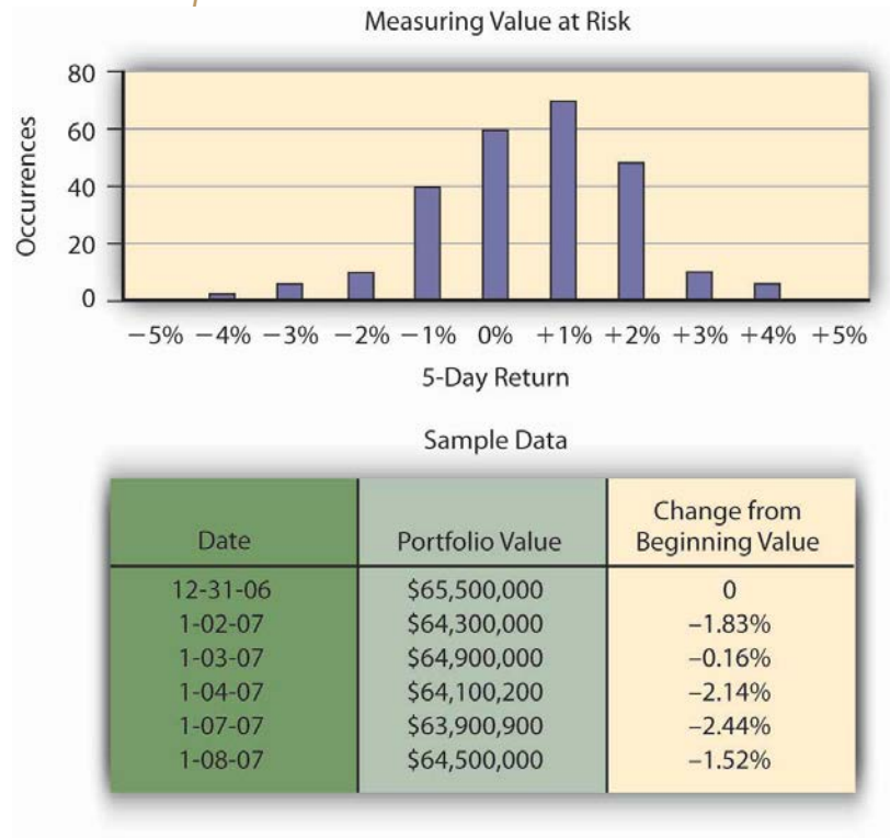
Figure 2.7 Hometown Bank Frequency Distribution of Daily Price Movement of Investment Securities Portfolio
