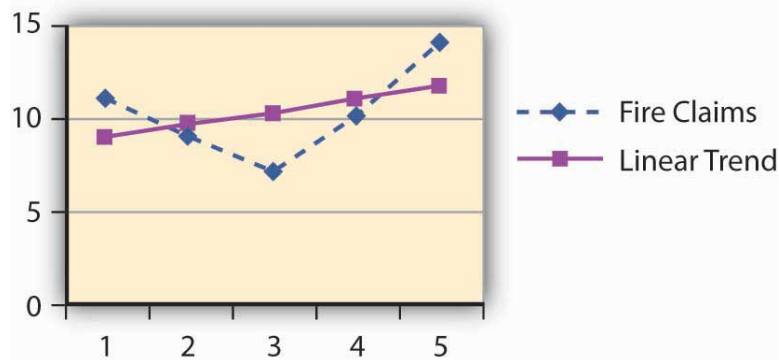
Figure 4.5 Linear Regression Trend of Claims of A
