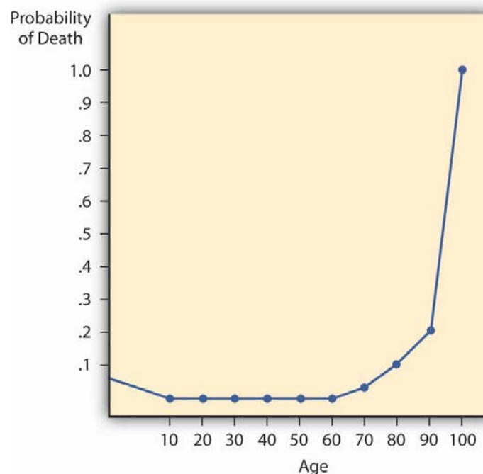
Figure 7.2 Male Mortality Curve
