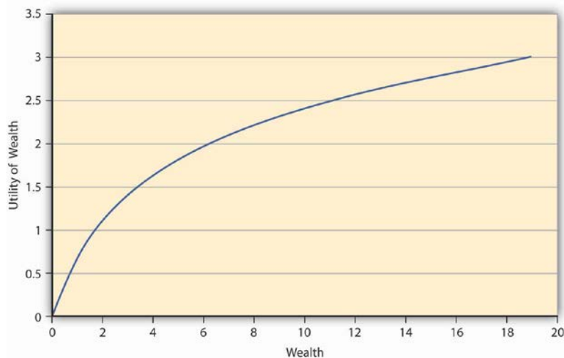
Figure 3.2 A Utility Function for a Risk-Averse Individual
