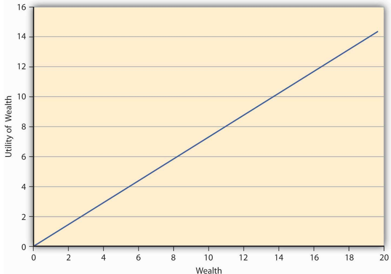
Figure 3.4 A Utility Function for a Risk-Neutral Individual
