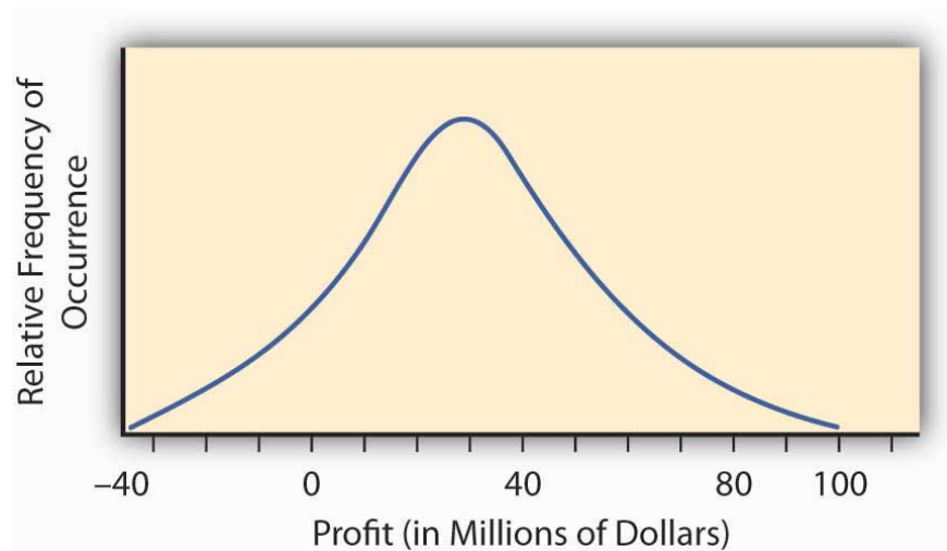
Figure 2.3 Normal Distribution of Potential Profit from a Research and Development Project
