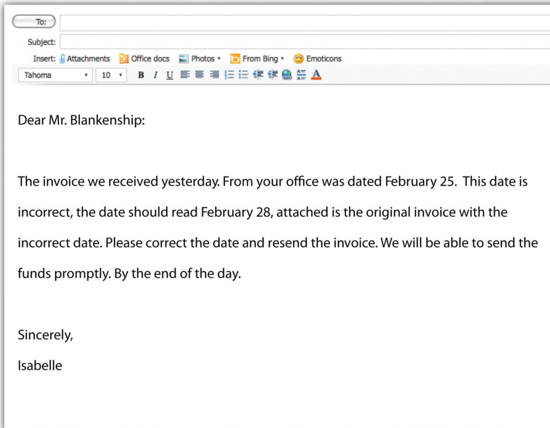
Figure 1.4 Sample e-mail
