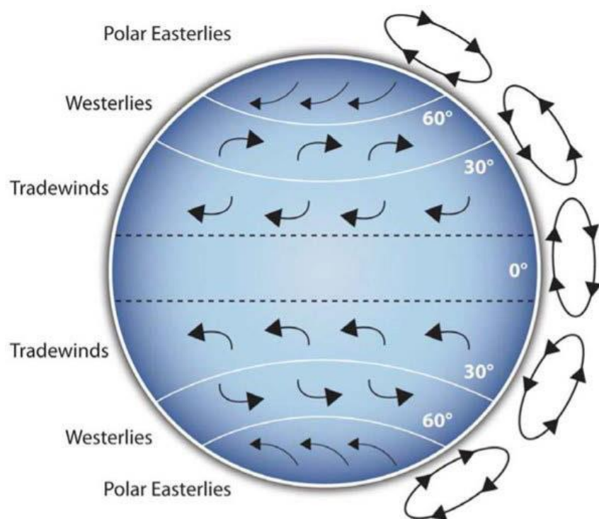
Figure 9.1 - Coriolis Effect
