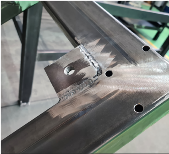
Fig.10/07 Welding is suitable for demanding applications, such as lug joints.
