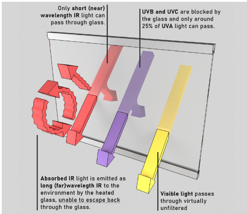
Fig.08/02 Illustration of the greenhouse effect.
