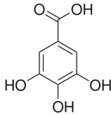
Figure 12.714 Structure of gallic acid, a polyphenol 5
