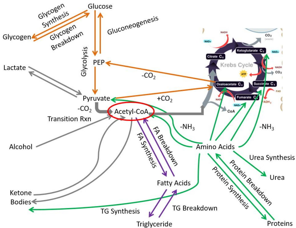
Figure 10.63 Acetyl-CoA is a central point in metabolism, and contains \text{CoA}^4
