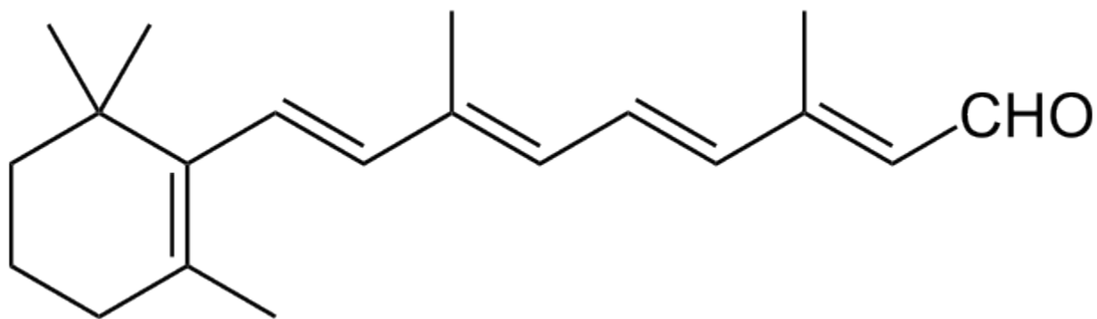
Retinal
