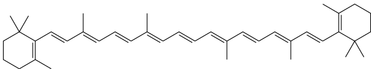
\beta -carotene
