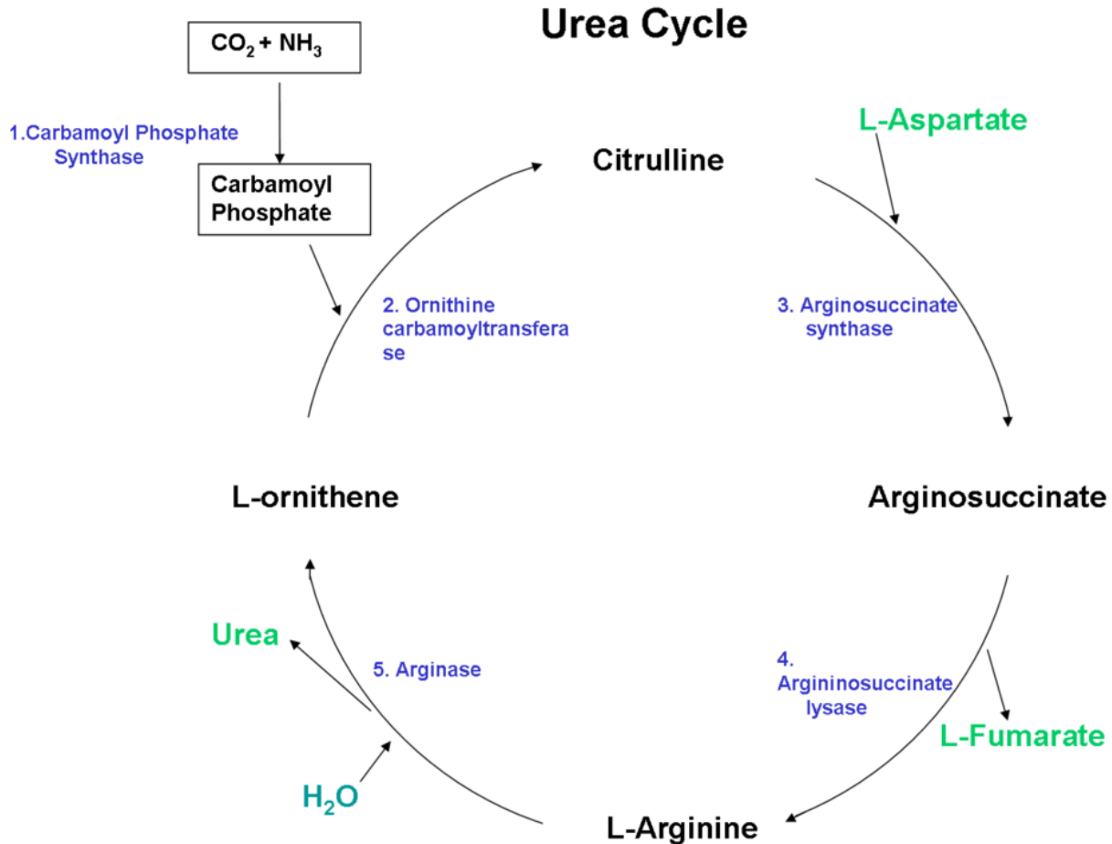
Figure 11.2: Urea cycle
