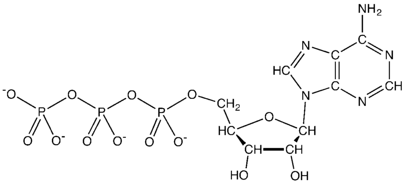
Figure 5.1: ATP structure
