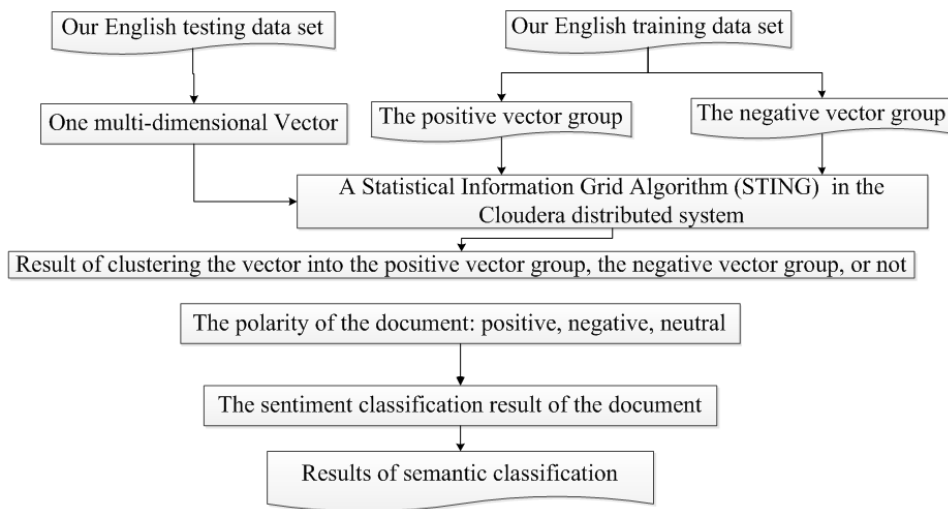
Fig. 6: A Statistical Information Grid Algorithm (STING) in the Parallel Network Environment
